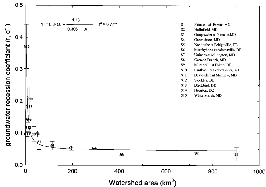
Figure 10. Hyperbolic relationship between the groundwater recession coefficient ( r , d^{-1} ) and watershed size ( km^2 ) for selected watersheds in the mid-Atlantic coastal plain region. Three hydrographs were analyzed for each watershed; data source = USGS.
