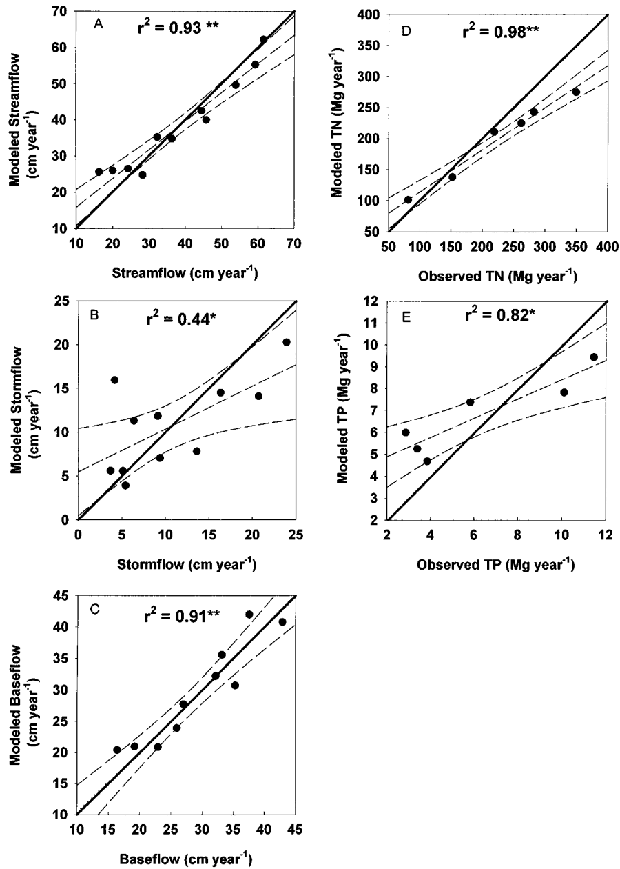
Figure 4. Correlations between modeled and observed annual measurements during the calibration period from WY1980–WY1990 at the Greensboro watershed. Solid line is the 1:1 line; dashed lines represent the line of best fit with 95% confidence limits.
