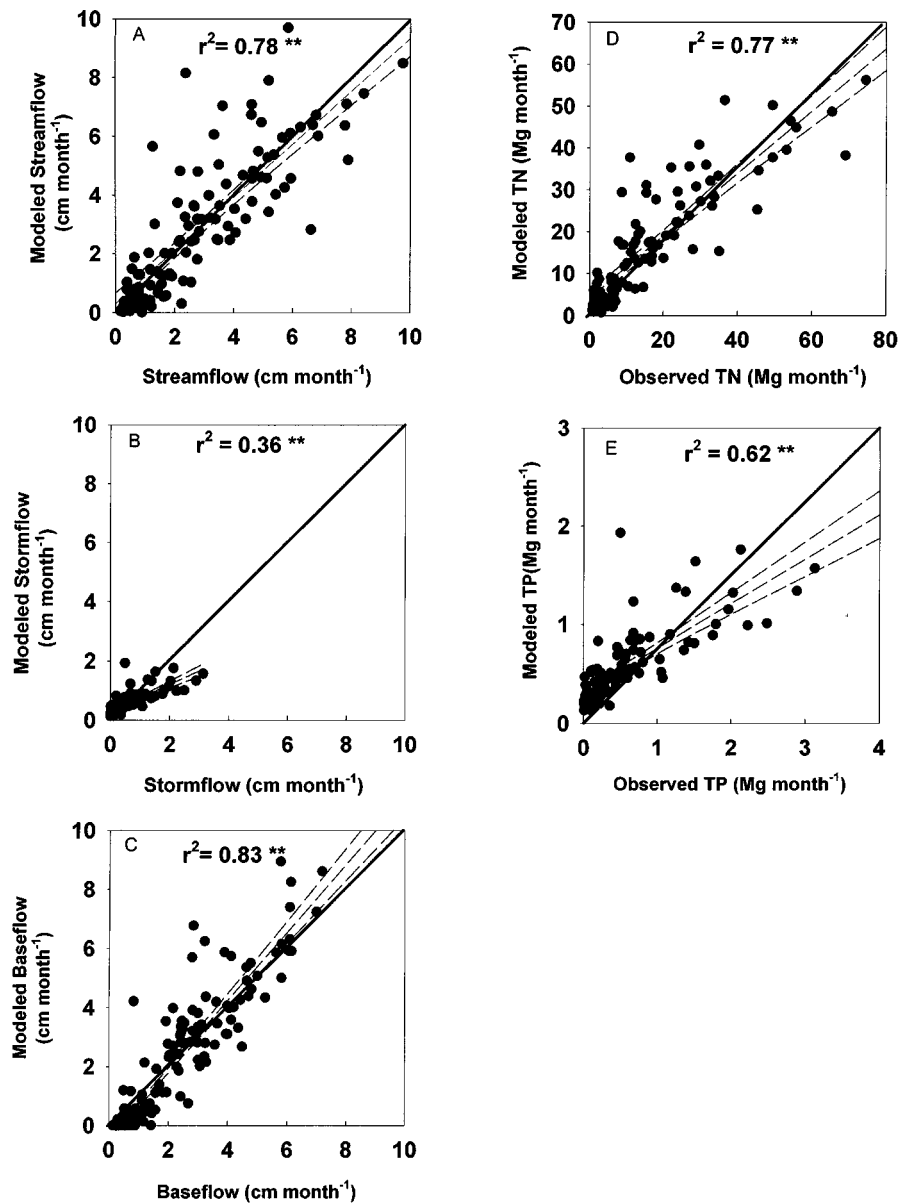
Figure 5. Correlations between modeled and observed monthly measurements during the calibration period from WY1980–WY1990 at the Greensboro watershed. Solid line is the 1:1 line; dashed lines represent the line of best fit with 95% confidence limits.
