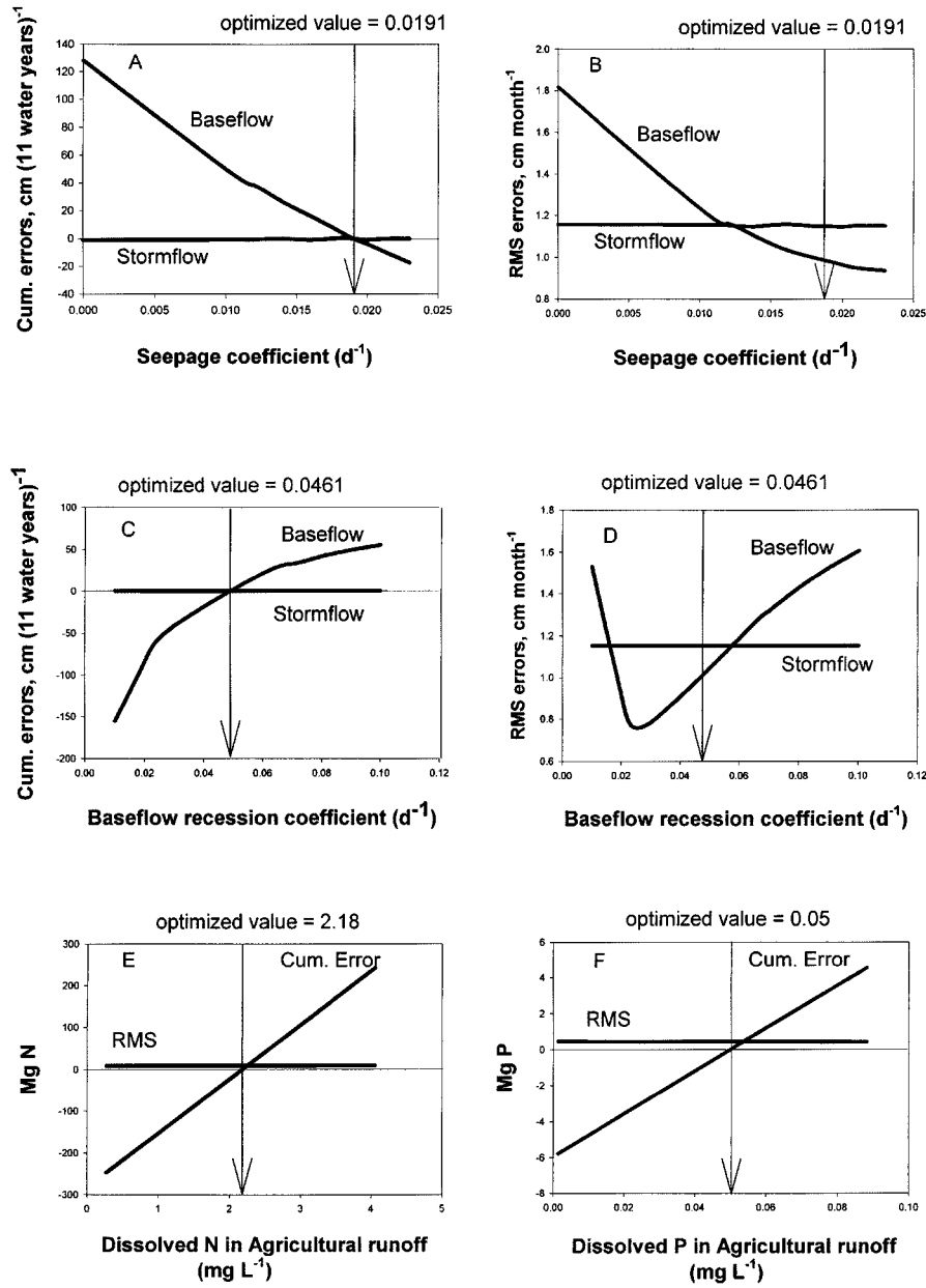
Figure 2. The optimization procedure employed to minimize cumulative and RMS errors for the seepage coefficient (A, B) and baseflow recession coefficient (C, D). Both coefficients primarily influence baseflow, with only minimal effects on stormflow. Arrows represent the optimized values for each parameter, chosen to minimize cumulative errors (A, C); the resulting RMS errors are shown in the B, D. Panels E, F indicate the selection of optimized values for dissolved N and P in agricultural stormflow. The units used for cumulative errors and RMS errors in the bottom panels are Mg (11 water years) -1 and Mg month -1 , respectively (Mg = 10 6 g).
