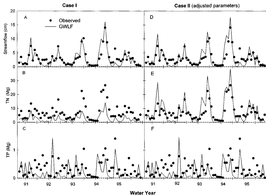
Figure 9. Model validation: time series of measurements at German Branch 310 with streamflow and N and P modeled with GWLF. Export modeled with GWLF is shown as solid lines; measurements from Jordan et al. (1997) are points. Simulations without local adjustments are shown in panels A, B, C (Case I); simulations with adjustments for local characteristics are shown in panels D, E, F (Case II).
