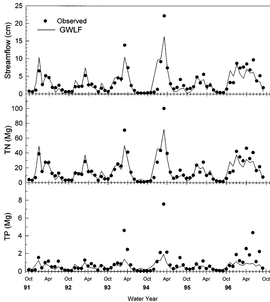
Figure 6. Model validation: time series comparisons of measurements by USGS at Greensboro compared with streamflow and export of N and P modeled with GWLF.
