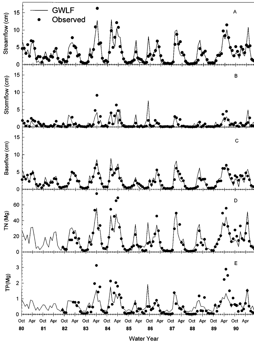
Figure 3. Time-series of observed monthly means at the gauged Greensboro subbasin compared with discharge and export of N and P modeled with GWLF. Export modeled with GWLF is shown as lines; observed data (Fisher et al. 1998) are points.
