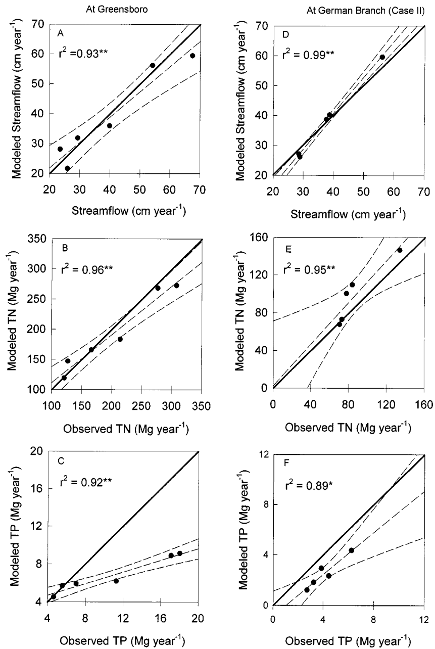
Figure 7. Correlations between modeled and observed annual measurements at Greensboro from WY1991–WY1996 and at German Branch 310 from WY1991–1995 (Case II). Solid line is the 1:1 line; dashed lines represent the line of best fit with 95% confidence limits.
