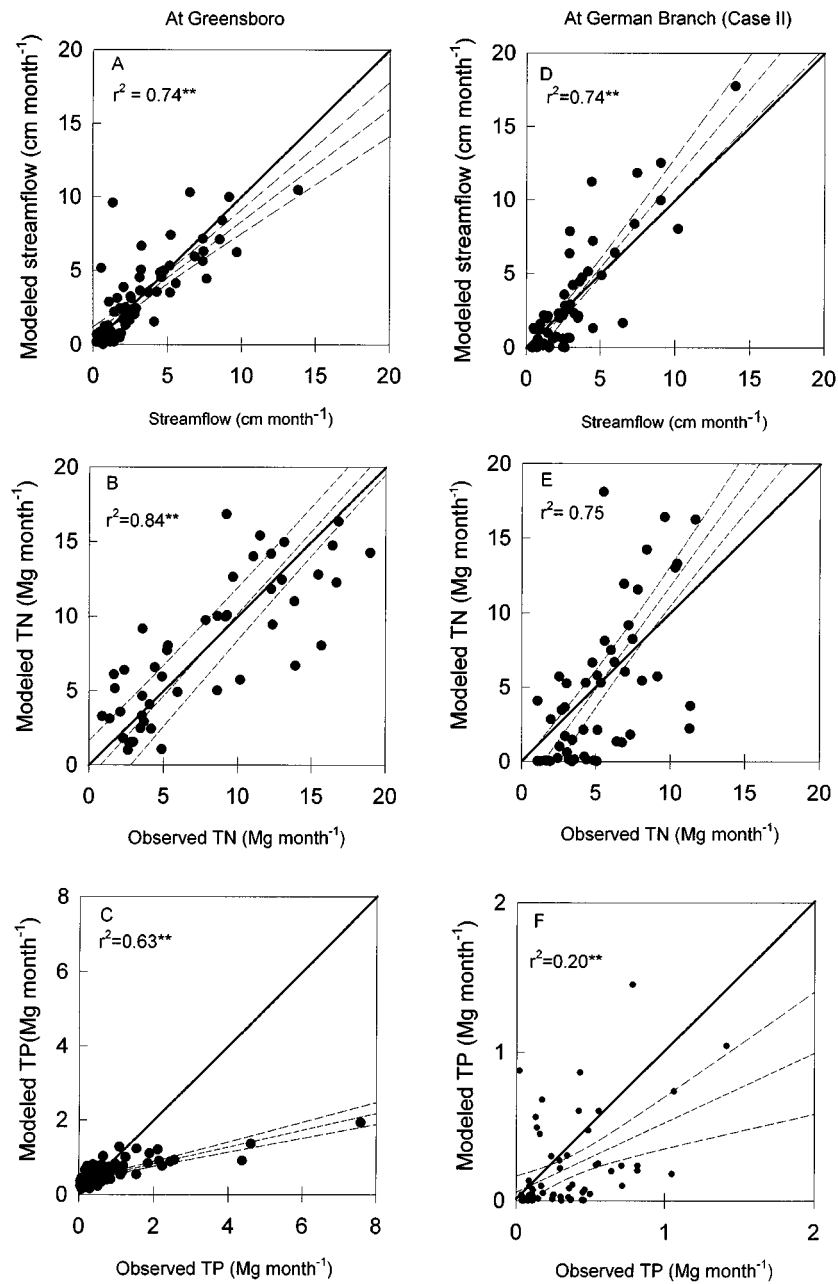
Figure 8. Correlations between modeled and observed monthly measurements at Greensboro from WY1991–WY1996 and at German Branch 310 from WY1991–1995 (Case II). Solid line is the 1:1 line; dashed lines represent the line of best fit with 95% confidence limits.
